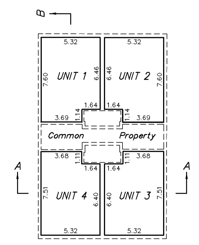
FIRST FLOOR SCALE = 1 : 200
